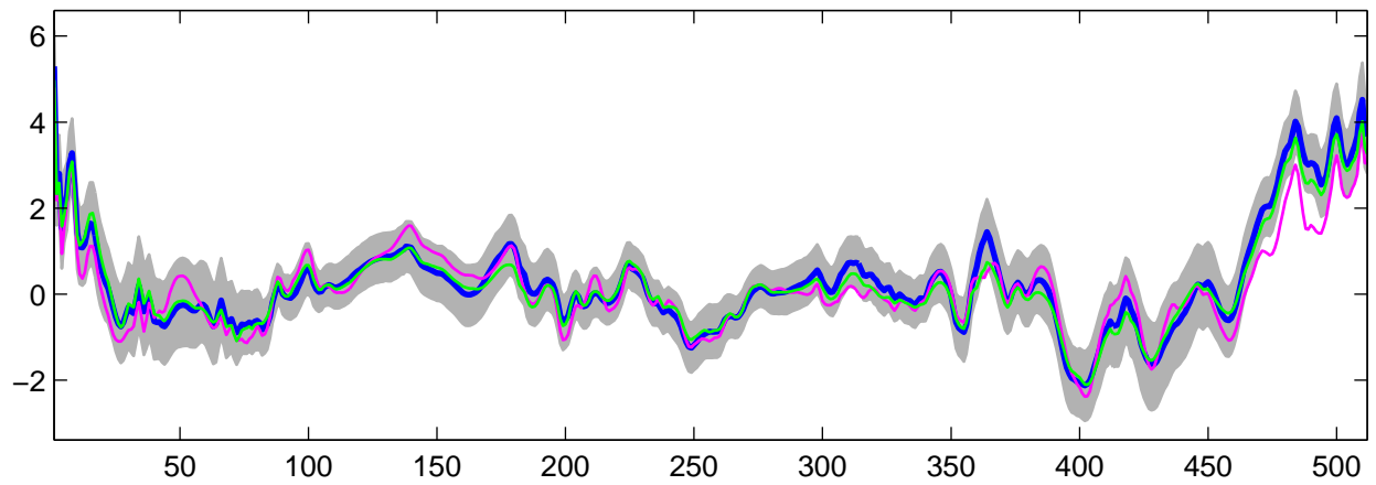
Estimated U_{14}(t) using R-WFMM: Normal data, run 10
