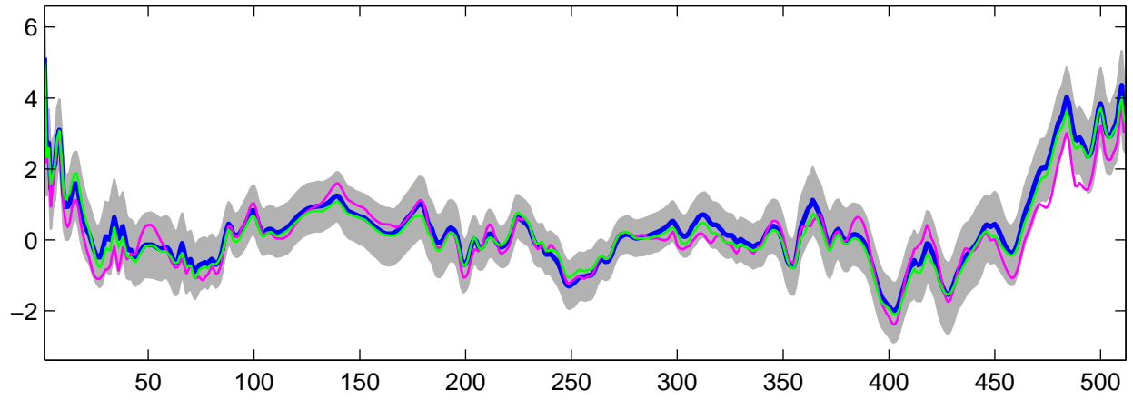
Estimated U_{14}(t) using G-WFMM: Normal data, run 10
