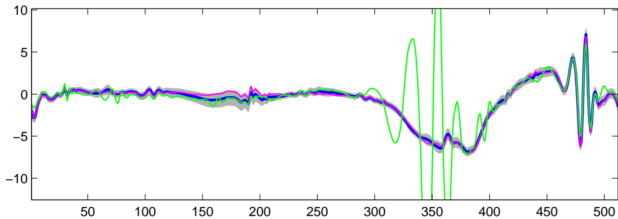
Estimated U_{14}(t) using R-WFMM: t_1 data, run 10
