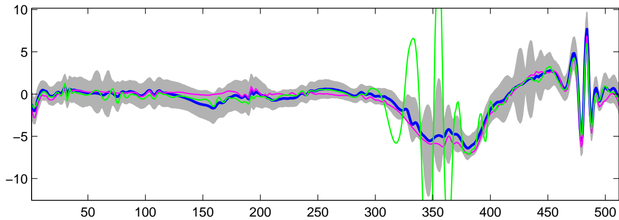
Estimated U_{14}(t) using G-WFMM: t_1 data, run 10
