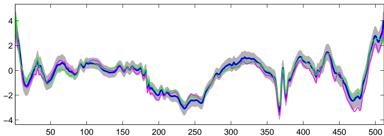
Estimated U_{14}(t) using R-WFMM: t_2 data, run 10
