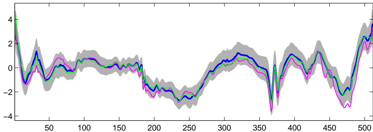
Estimated U_{14}(t) using G-WFMM: t_2 data, run 10
