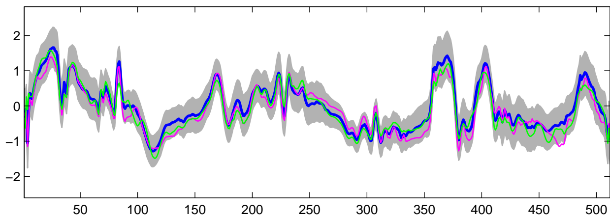
Estimated U_{14}(t) using R-WFMM: t_3 data, run 10
