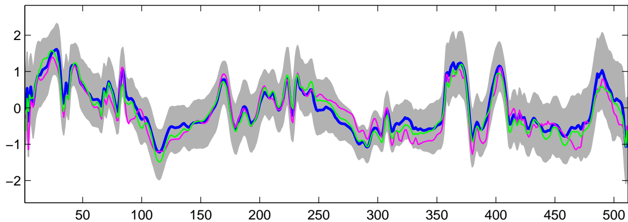
Estimated U_{14}(t) using G-WFMM: t_3 data, run 10
