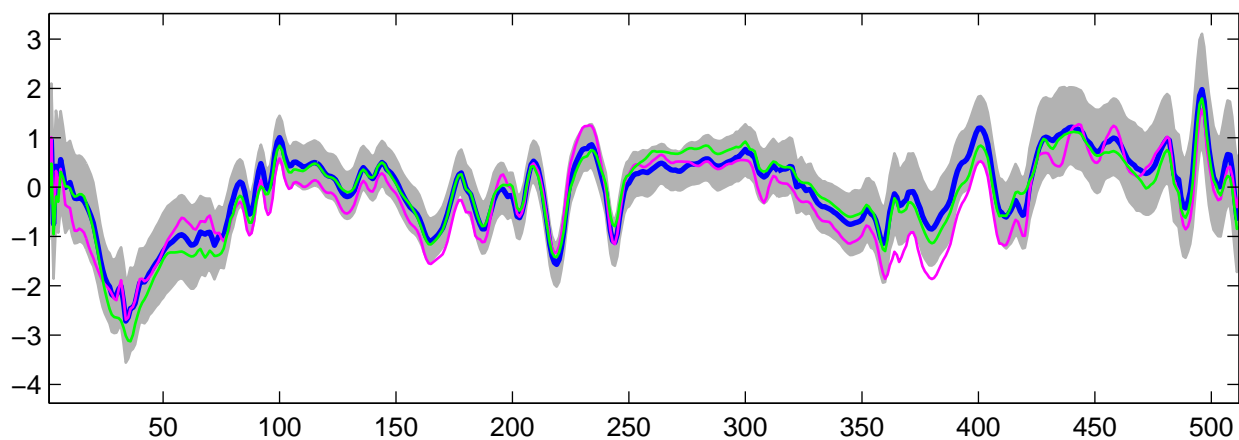
Estimated U_{15}(t) using R-WFMM: DE data, run 10
