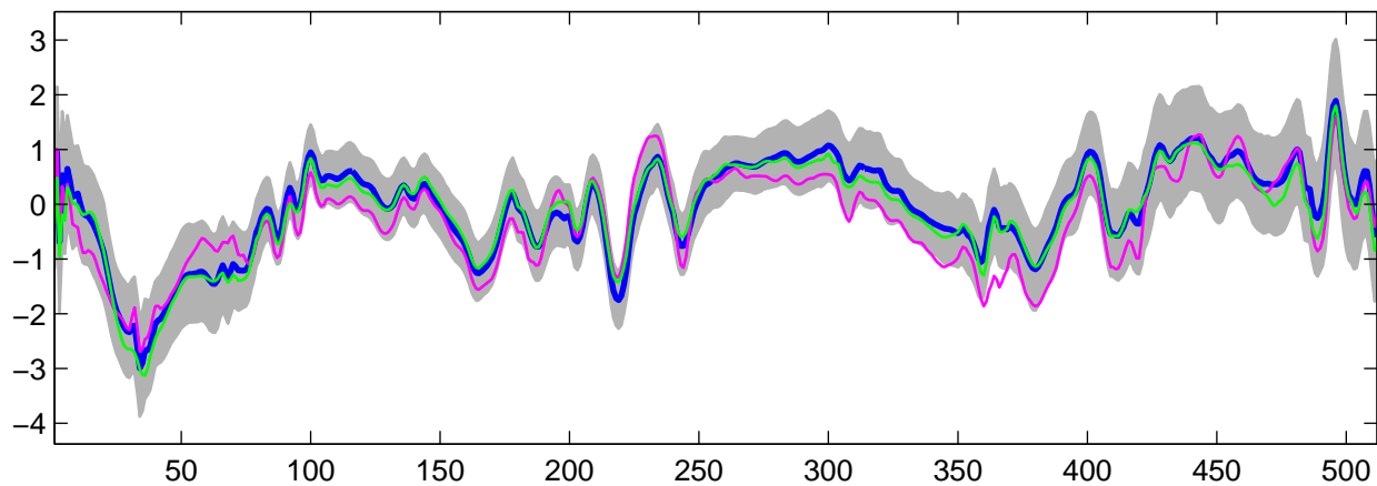
Estimated U_{15}(t) using G-WFMM: DE data, run 10
