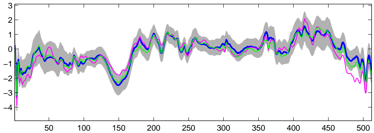
Estimated U_{15}(t) using R-WFMM: Normal data, run 10
