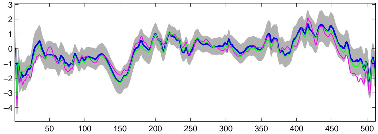
Estimated U_{15}(t) using G-WFMM: Normal data, run 10
