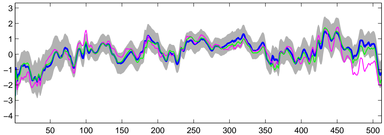
Estimated U_{16}(t) using R-WFMM: Normal data, run 10
