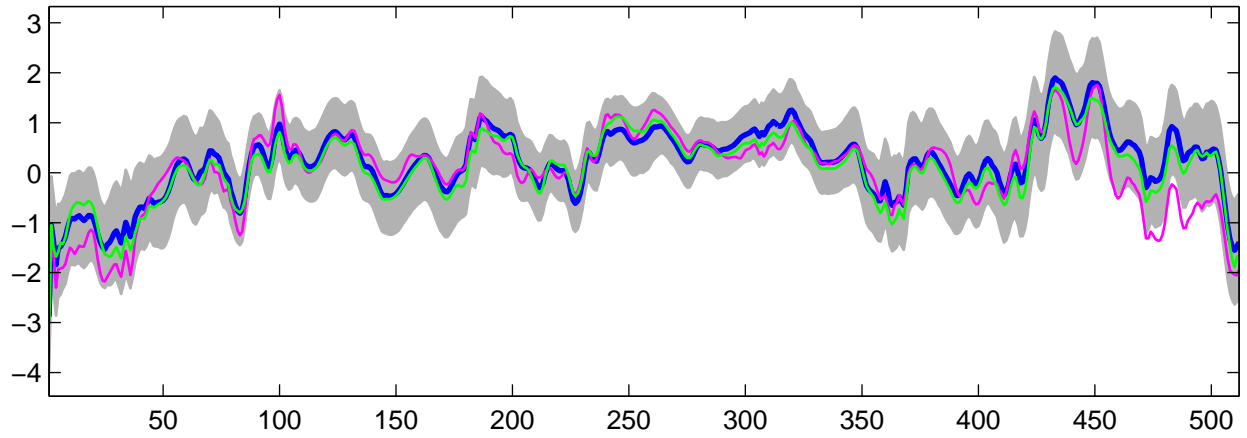
Estimated U_{16}(t) using G-WFMM: Normal data, run 10
