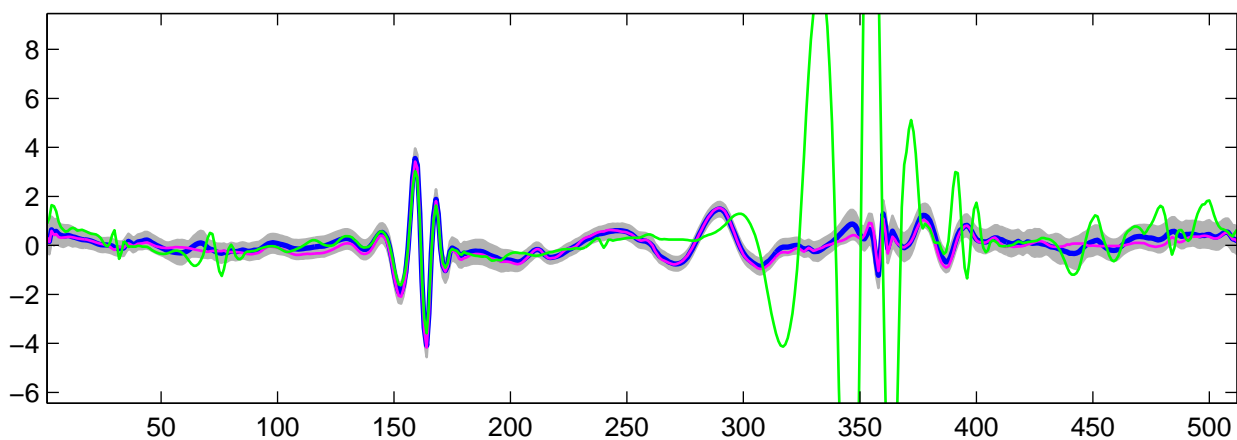
Estimated U_{16}(t) using R-WFMM: t_1 data, run 10
