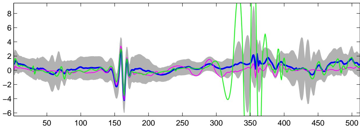
Estimated U_{16}(t) using G-WFMM: t_1 data, run 10
