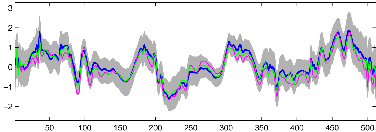
Estimated U_{16}(t) using G-WFMM: t_3 data, run 10
