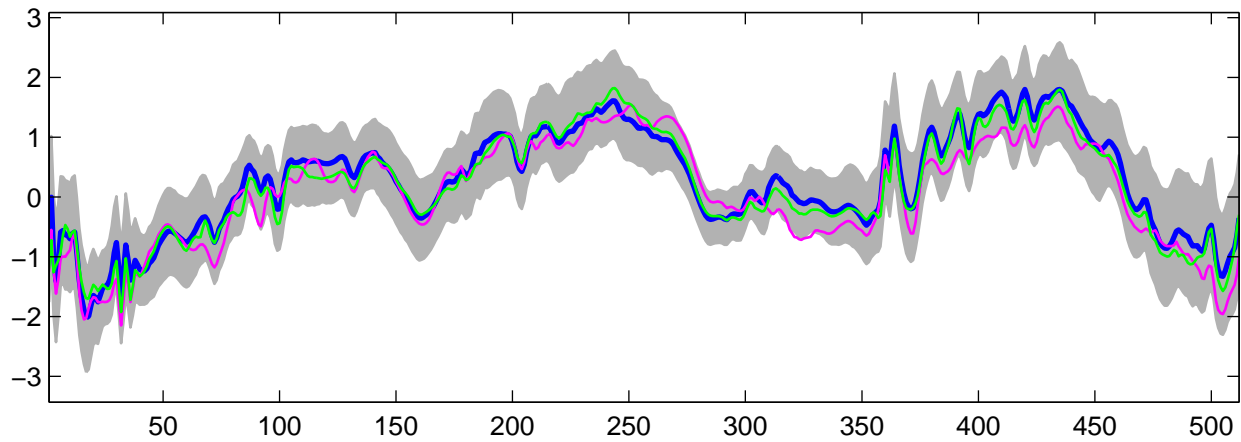
Estimated U_{17}(t) using G-WFMM: t_3 data, run 10
