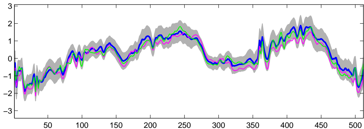
Estimated U_{17}(t) using R-WFMM: t_3 data, run 10
