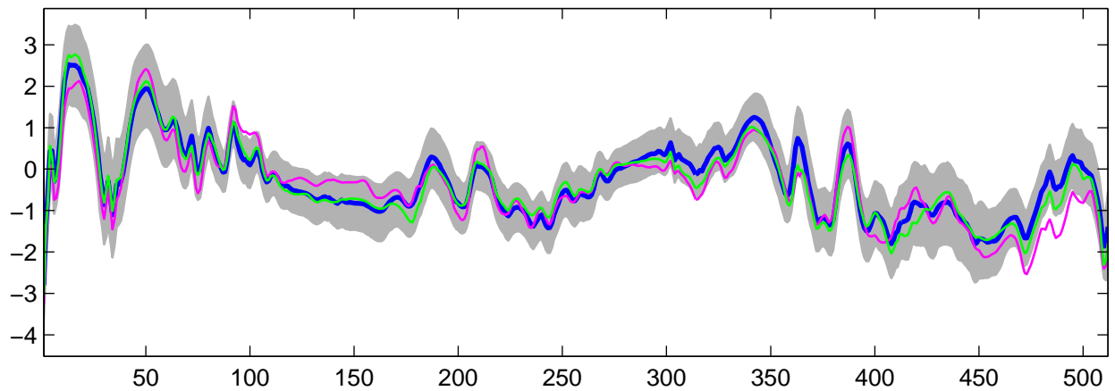
Estimated U_{18}(t) using R-WFMM: Normal data, run 10
