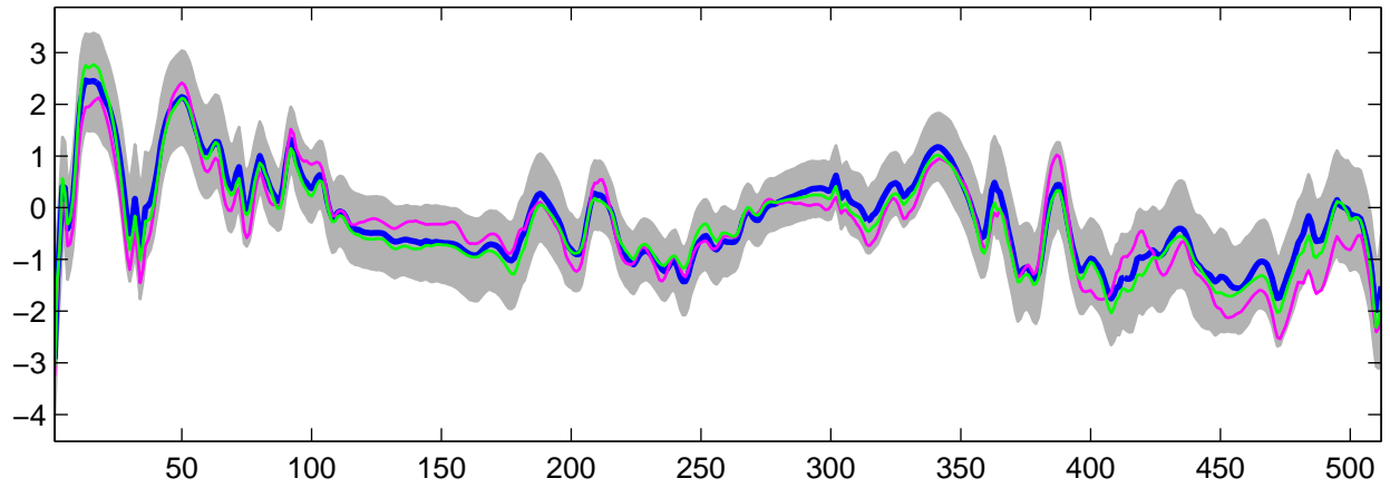
Estimated U_{18}(t) using G-WFMM: Normal data, run 10
