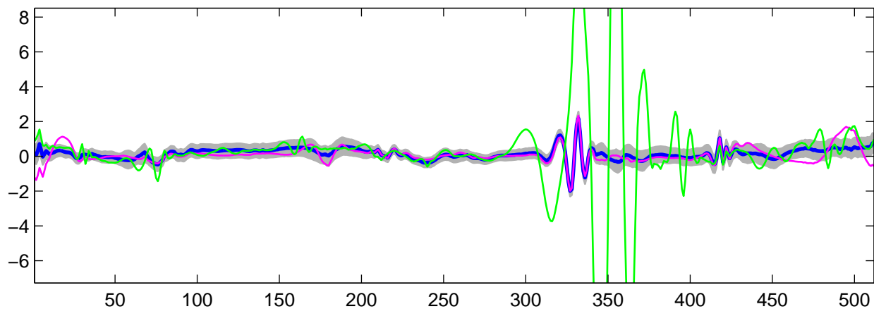
Estimated U_{18}(t) using R-WFMM: t_1 data, run 10
