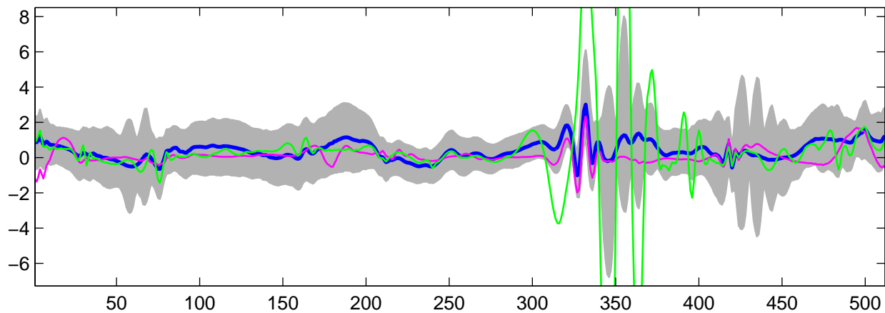
Estimated U_{18}(t) using G-WFMM: t_1 data, run 10
