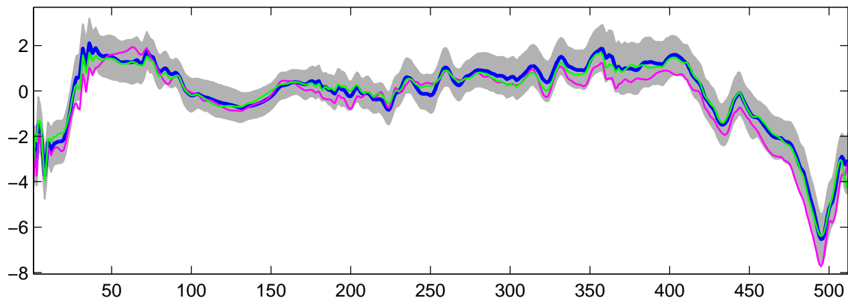
Estimated U_{18}(t) using G-WFMM: t_2 data, run 10
