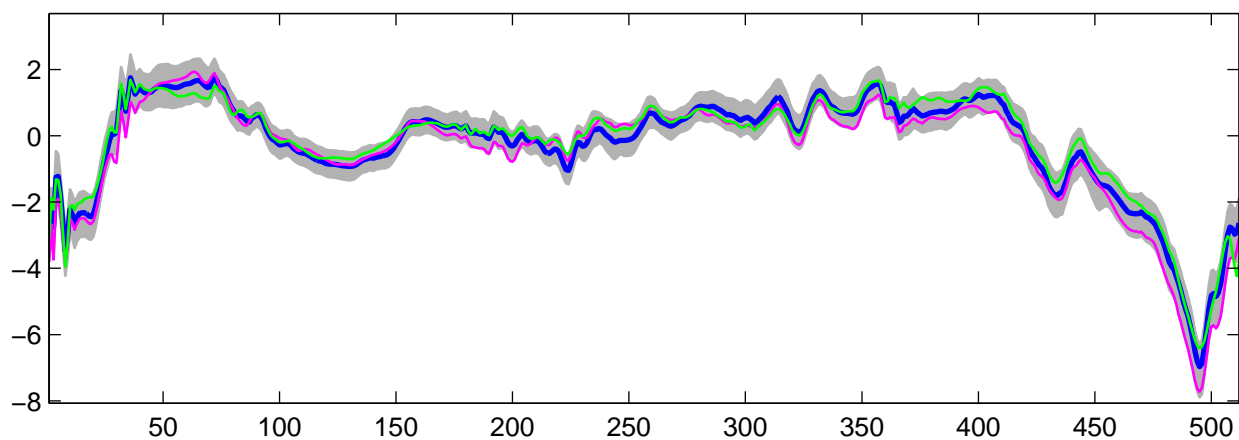
Estimated U_{18}(t) using R-WFMM: t_2 data, run 10
