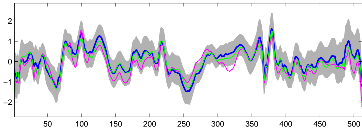
Estimated U_{18}(t) using G-WFMM: t_3 data, run 10
