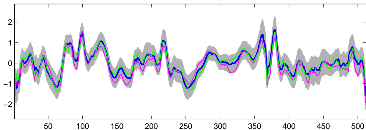
Estimated U_{18}(t) using R-WFMM: t_3 data, run 10
