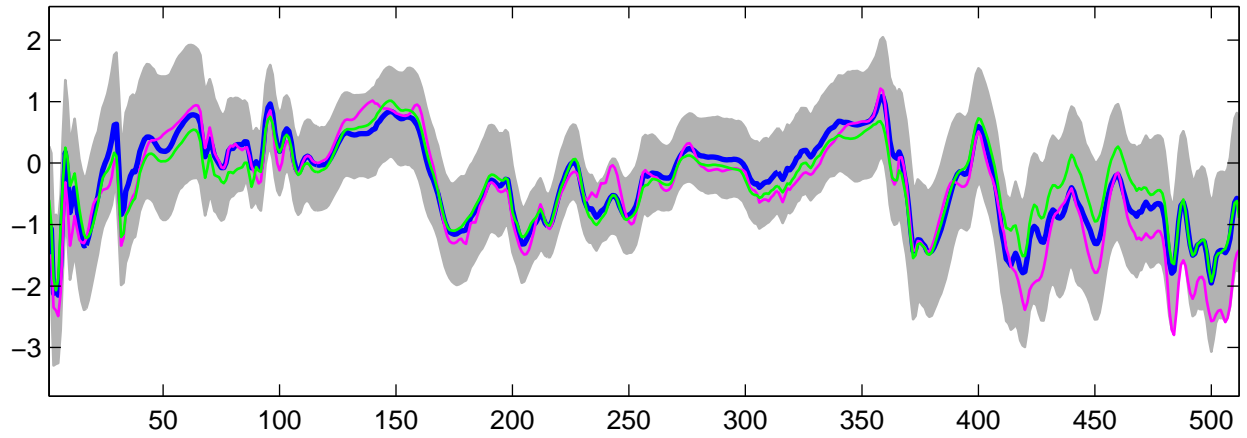
Estimated U_{19}(t) using G-WFMM: Normal data, run 10
