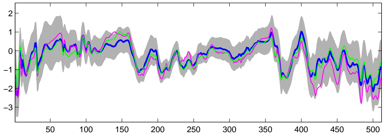
Estimated U_{19}(t) using R-WFMM: Normal data, run 10
