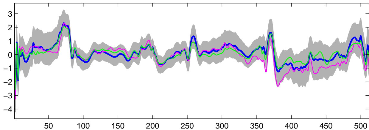
Estimated U_{19}(t) using G-WFMM: t_2 data, run 10
