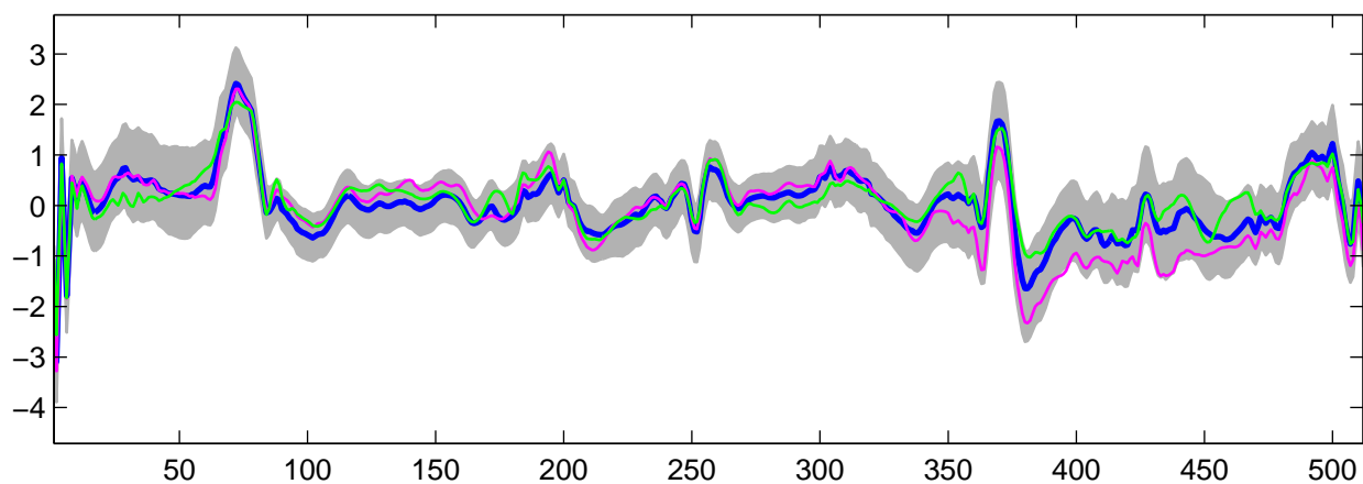
Estimated U_{19}(t) using R-WFMM: t_2 data, run 10
