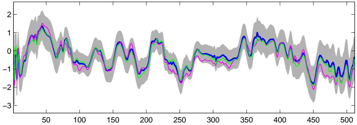
Estimated U_1(t) using G-WFMM: Normal data, run 10
