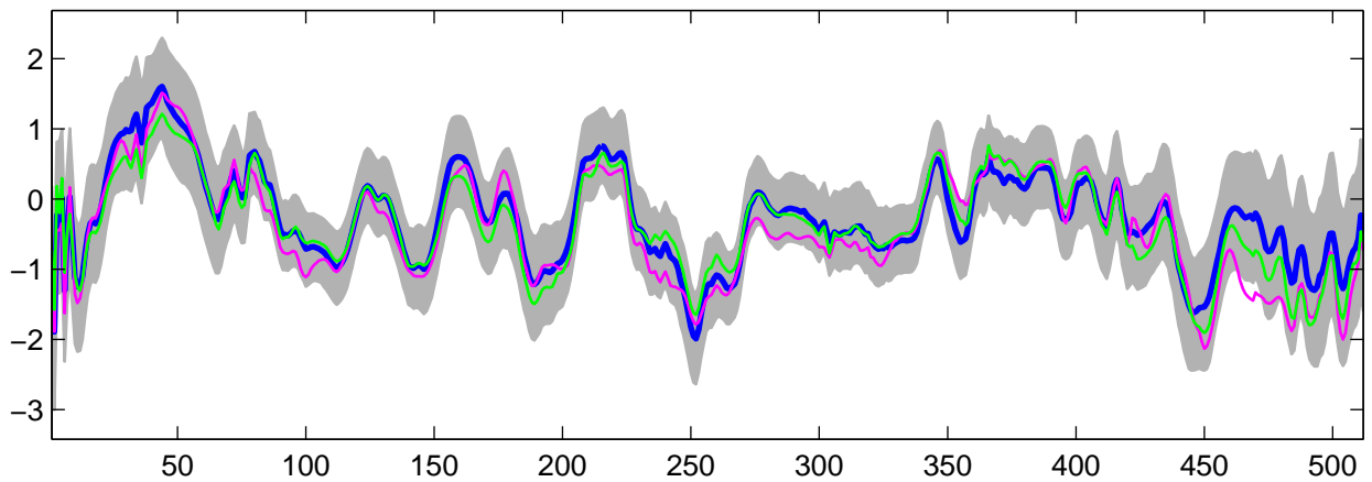
Estimated U_1(t) using R-WFMM: Normal data, run 10
