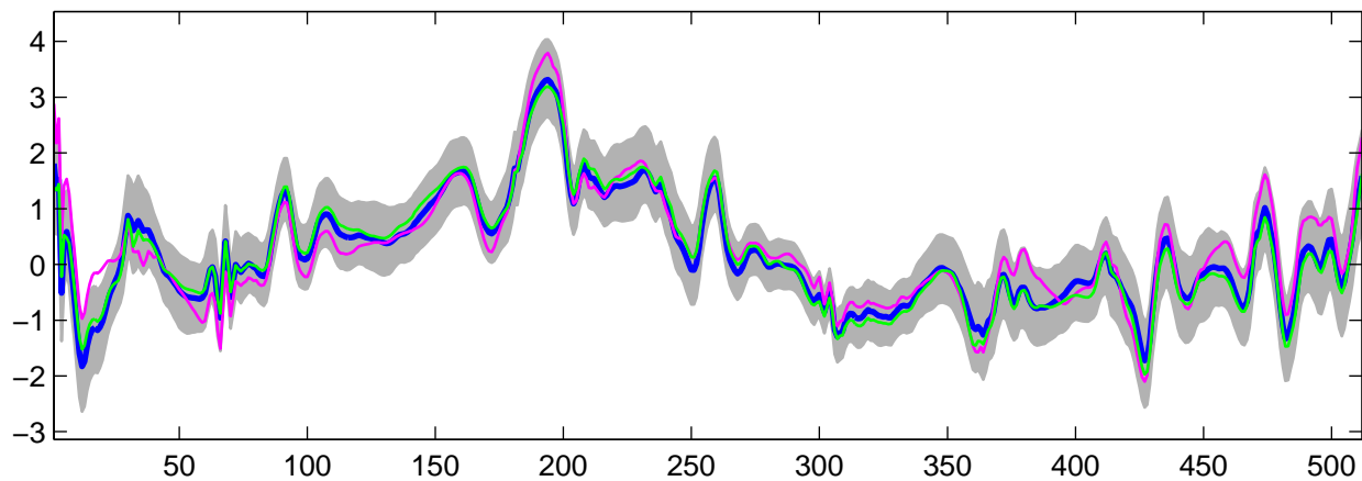
Estimated U_1(t) using G-WFMM: t_3 data, run 10
