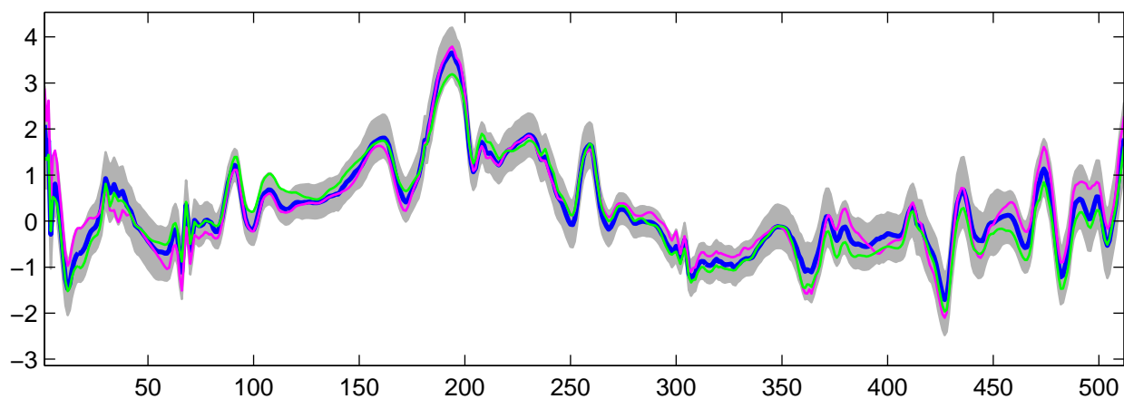
Estimated U_1(t) using R-WFMM: t_3 data, run 10
