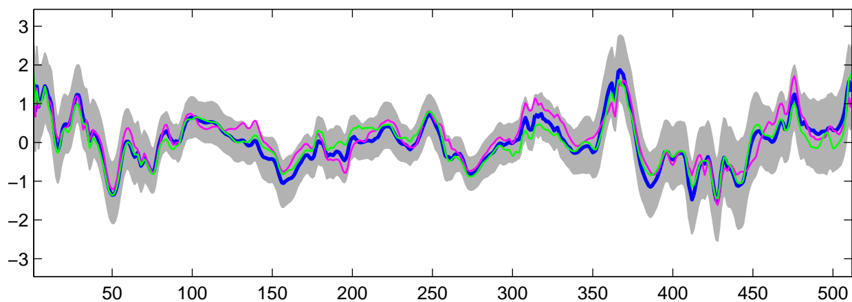
Estimated U_{20}(t) using R-WFMM: DE data, run 10
