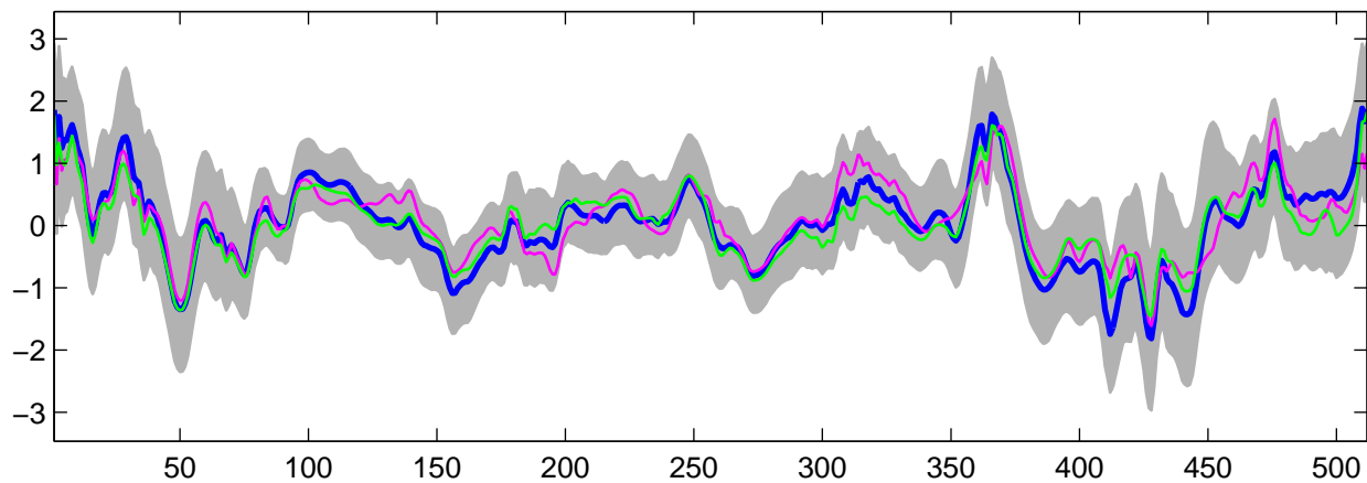
Estimated U_{20}(t) using G-WFMM: DE data, run 10
