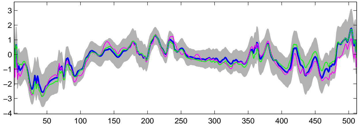
Estimated U_{20}(t) using G-WFMM: Normal data, run 10
