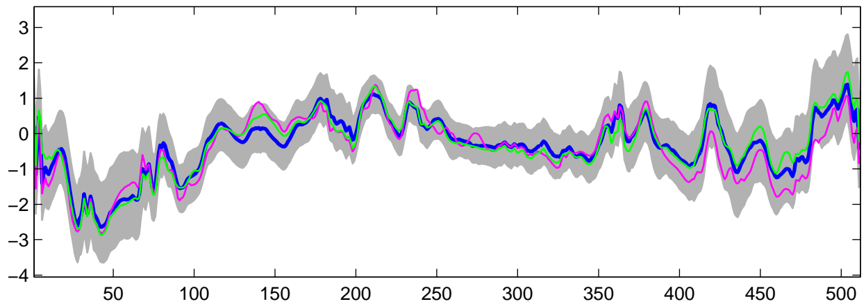
Estimated U_{20}(t) using R-WFMM: Normal data, run 10
