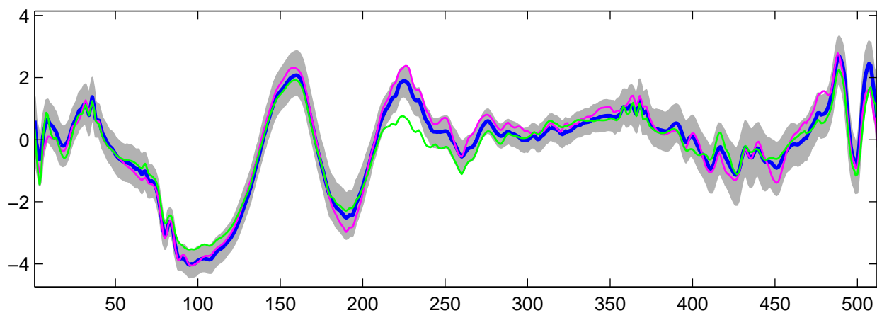
Estimated U_{20}(t) using R-WFMM: t_3 data, run 10
