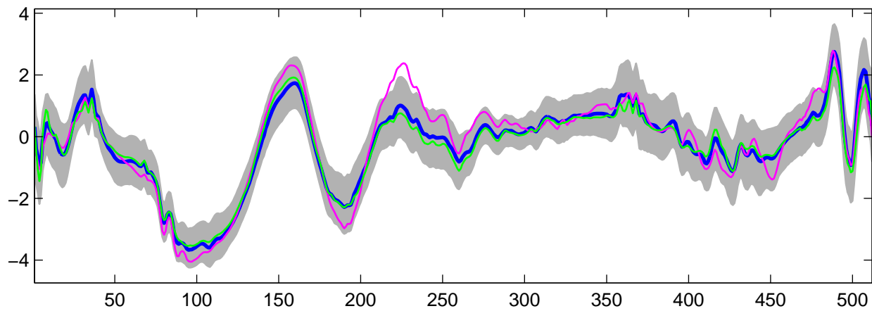
Estimated U_{20}(t) using G-WFMM: t_3 data, run 10
