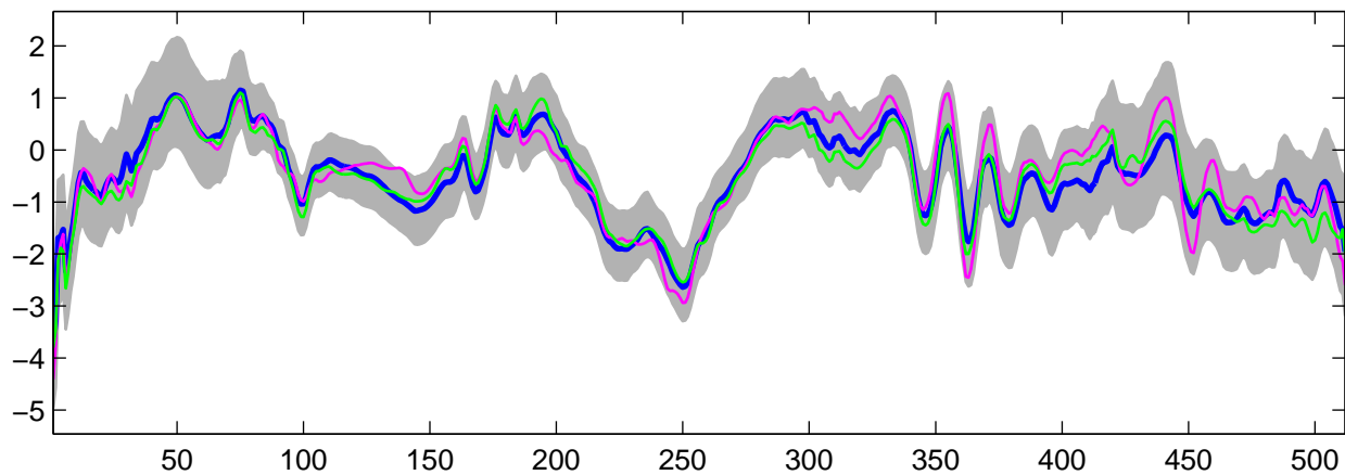
Estimated U_{21}(t) using G-WFMM: DE data, run 10
