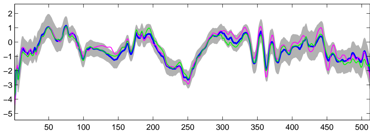
Estimated U_{21}(t) using R-WFMM: DE data, run 10
