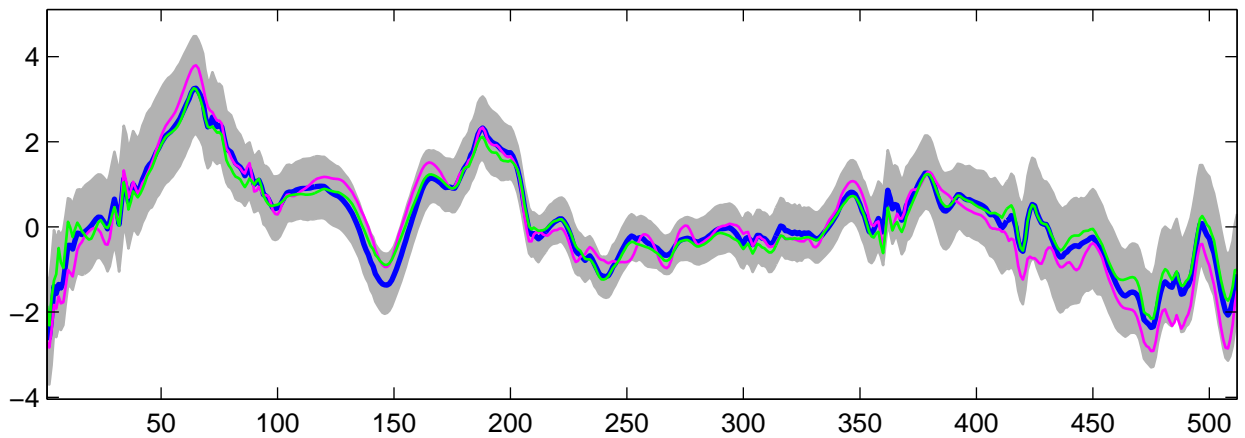
Estimated U_{21}(t) using R-WFMM: Normal data, run 10
