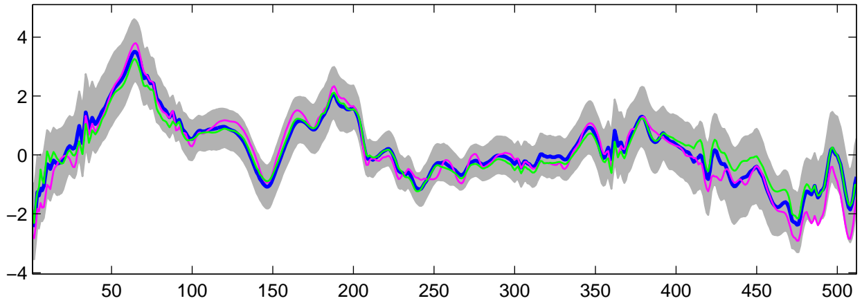
Estimated U_{21}(t) using G-WFMM: Normal data, run 10
