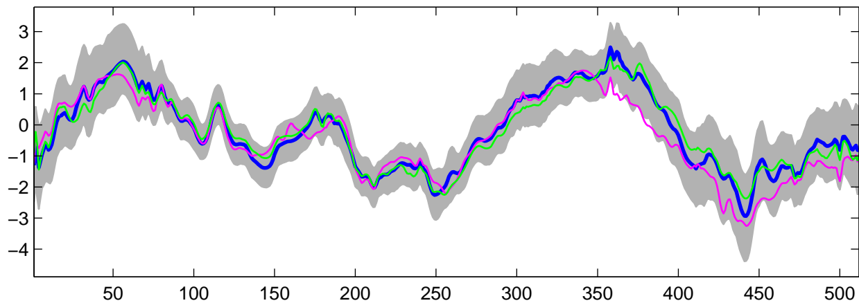
Estimated U_{21}(t) using G-WFMM: t_2 data, run 10
