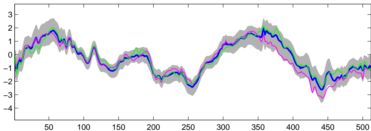
Estimated U_{21}(t) using R-WFMM: t_2 data, run 10
