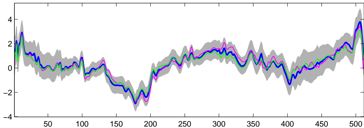
Estimated U_{22}(t) using G-WFMM: DE data, run 10
