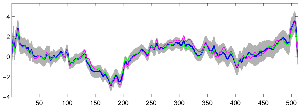
Estimated U_{22}(t) using R-WFMM: DE data, run 10
