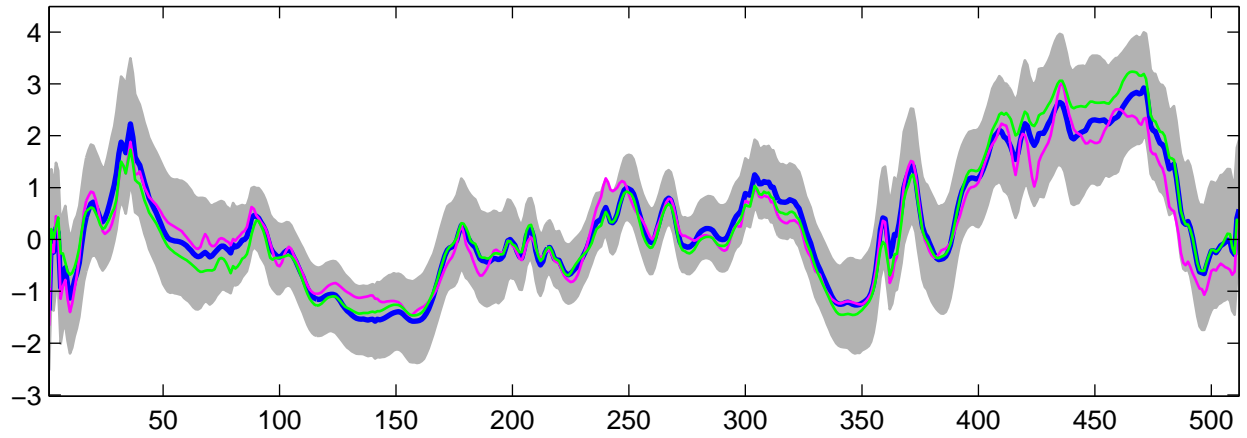
Estimated U_{22}(t) using G-WFMM: Normal data, run 10
