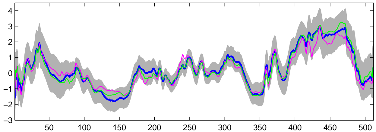
Estimated U_{22}(t) using R-WFMM: Normal data, run 10
