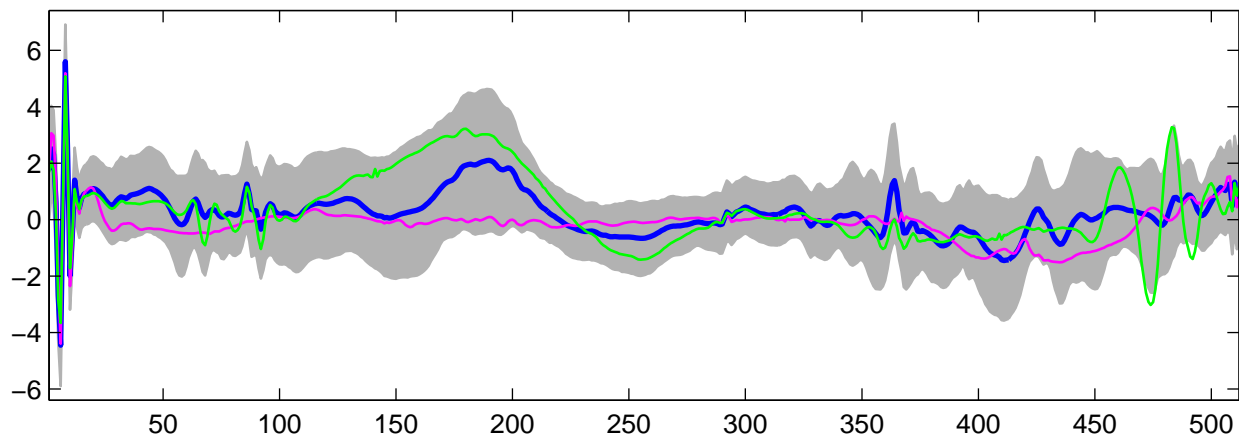
Estimated U_{22}(t) using G-WFMM: t_1 data, run 10
