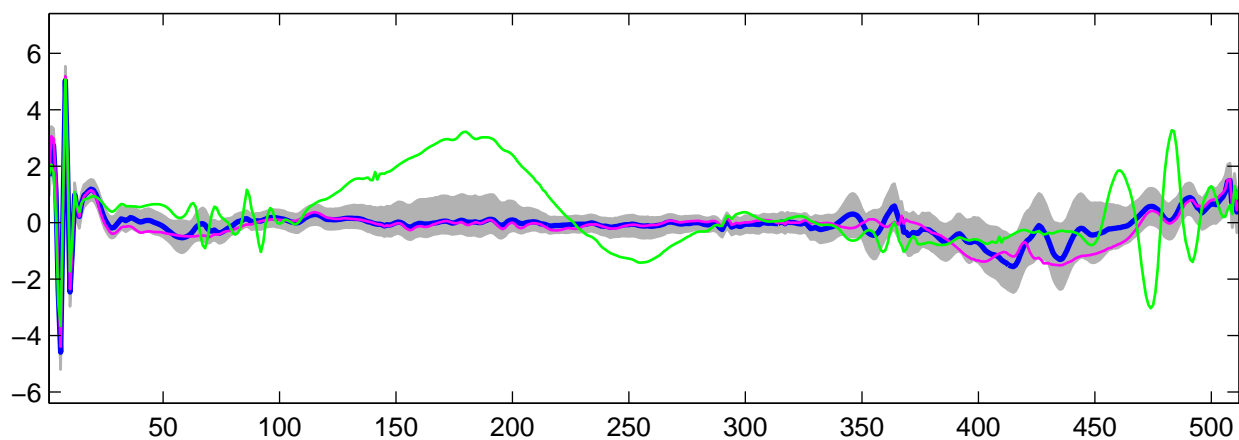
Estimated U_{22}(t) using R-WFMM: t_1 data, run 10
