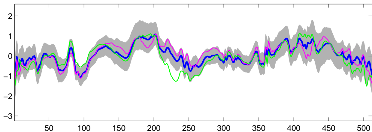
Estimated U_{22}(t) using R-WFMM: t_3 data, run 10
