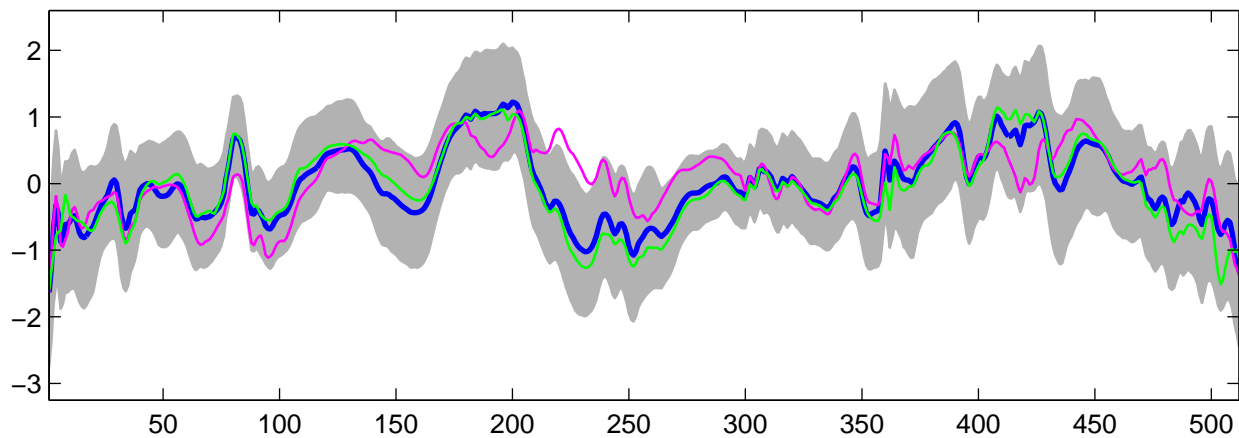
Estimated U_{22}(t) using G-WFMM: t_3 data, run 10
