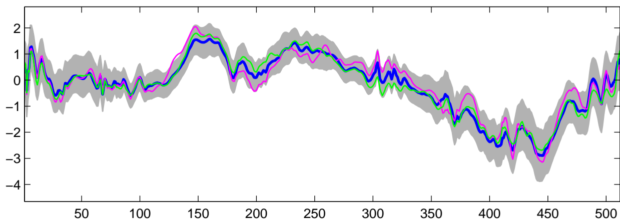
Estimated U_{23}(t) using R-WFMM: DE data, run 10
