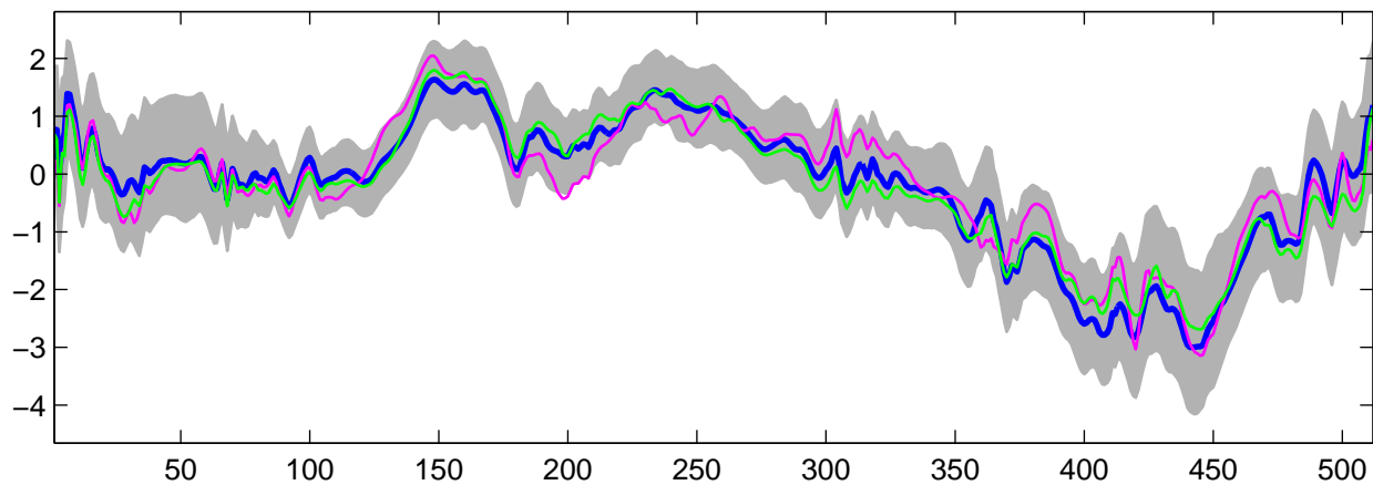
Estimated U_{23}(t) using G-WFMM: DE data, run 10
