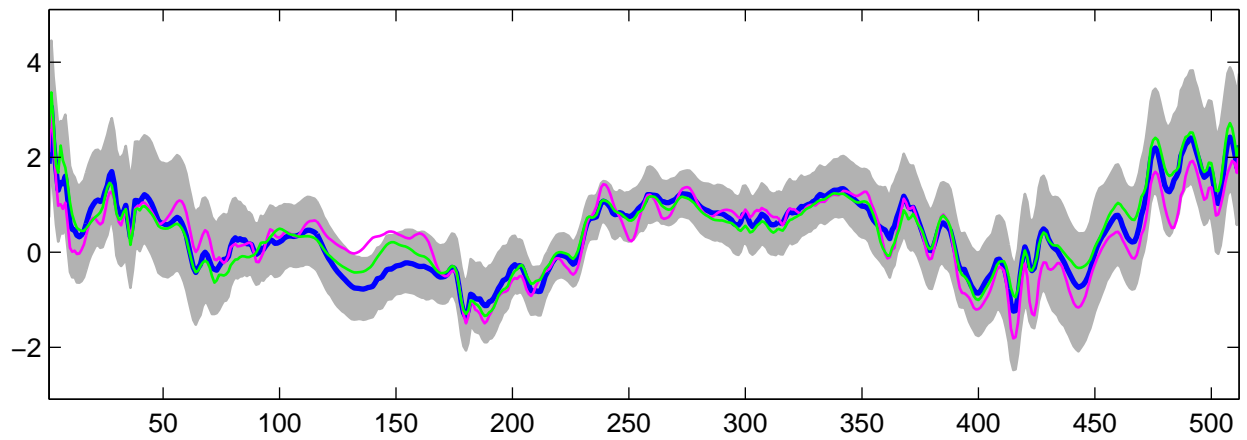
Estimated U_{23}(t) using R-WFMM: Normal data, run 10
