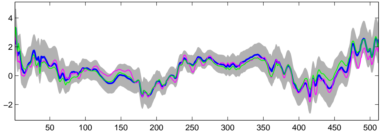
Estimated U_{23}(t) using G-WFMM: Normal data, run 10
