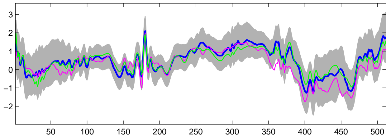
Estimated U_{23}(t) using G-WFMM: t_2 data, run 10
