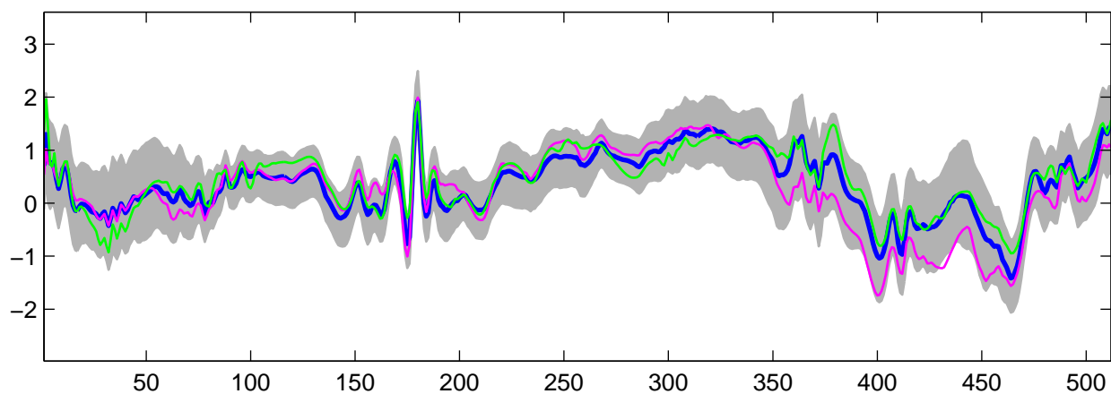
Estimated U_{23}(t) using R-WFMM: t_2 data, run 10
