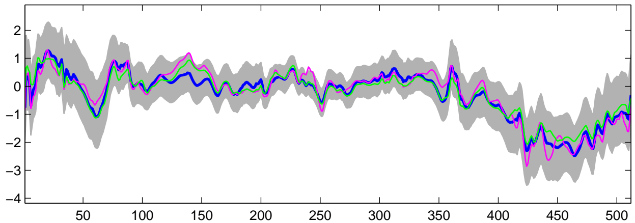
Estimated U_{24}(t) using R-WFMM: Normal data, run 10
