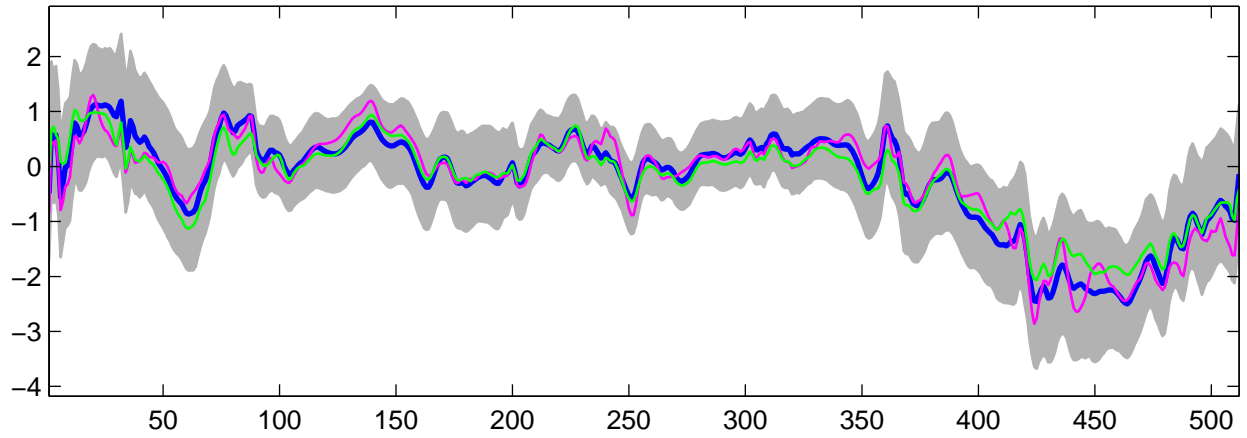
Estimated U_{24}(t) using G-WFMM: Normal data, run 10
