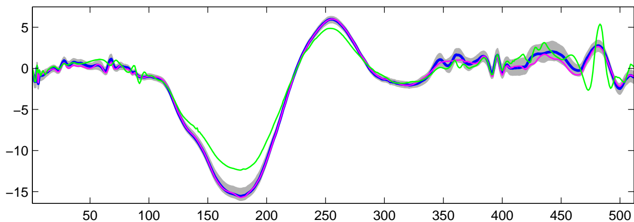
Estimated U_{24}(t) using R-WFMM: t_1 data, run 10
