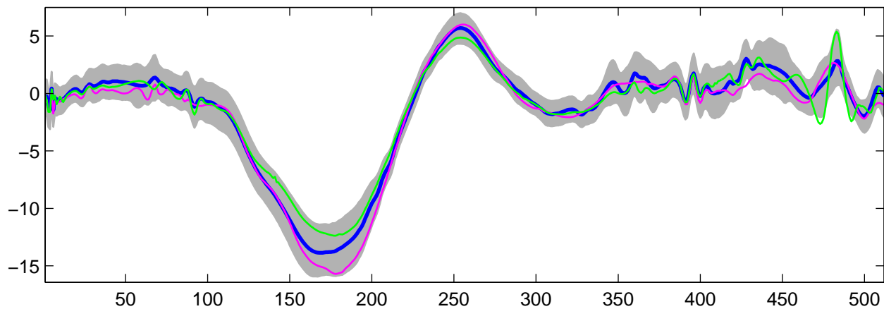
Estimated U_{24}(t) using G-WFMM: t_1 data, run 10
