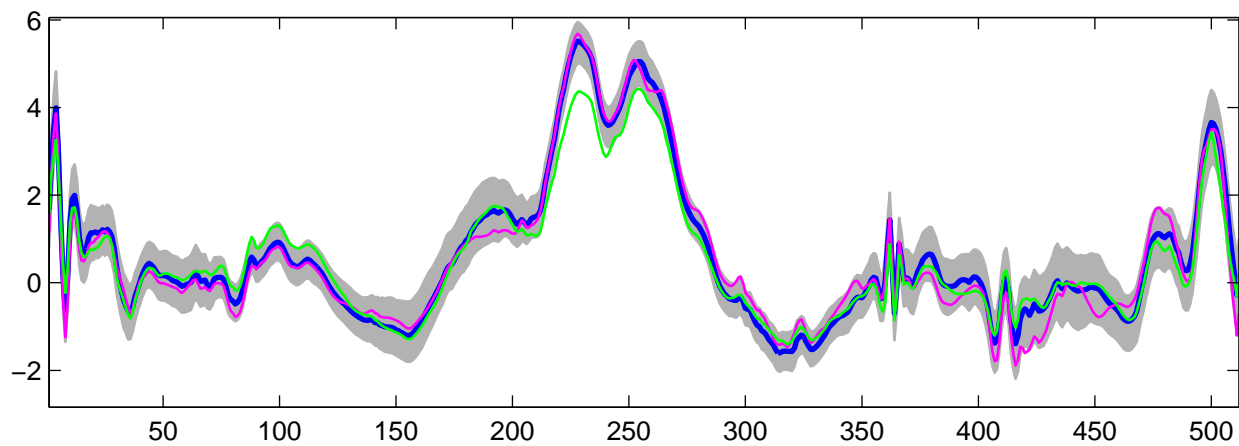
Estimated U_{24}(t) using R-WFMM: t_3 data, run 10
