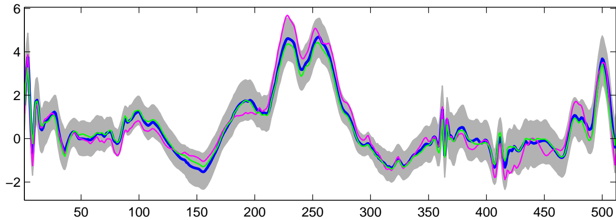
Estimated U_{24}(t) using G-WFMM: t_3 data, run 10
