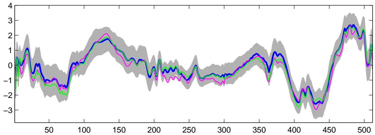
Estimated U_{25}(t) using R-WFMM: Normal data, run 10
