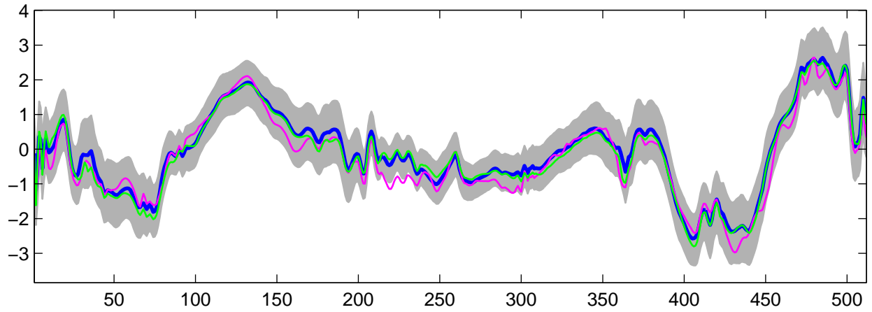
Estimated U_{25}(t) using G-WFMM: Normal data, run 10
