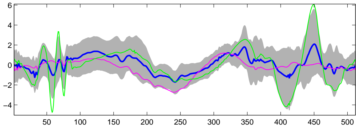
Estimated U_{25}(t) using G-WFMM: t_1 data, run 10
