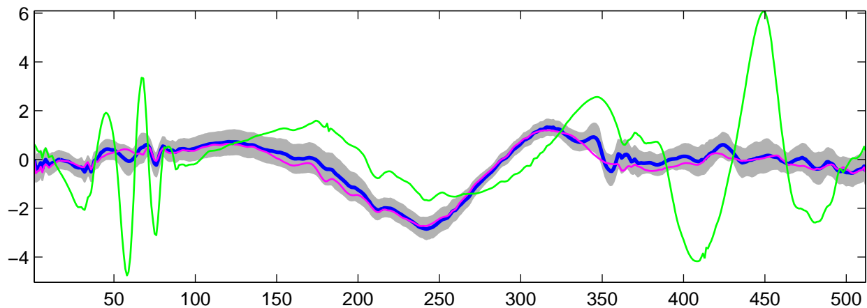
Estimated U_{25}(t) using R-WFMM: t_1 data, run 10
