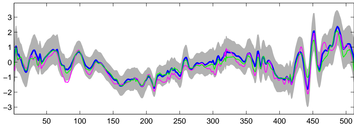
Estimated U_{25}(t) using G-WFMM: t_2 data, run 10
