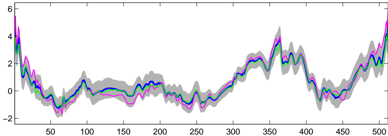
Estimated U_{25}(t) using G-WFMM: t_3 data, run 10
