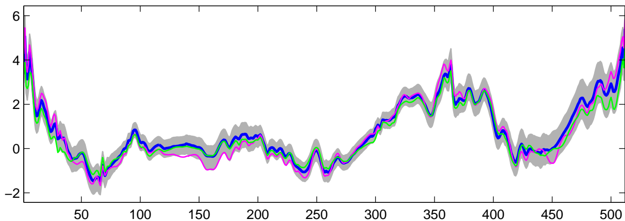
Estimated U_{25}(t) using R-WFMM: t_3 data, run 10
