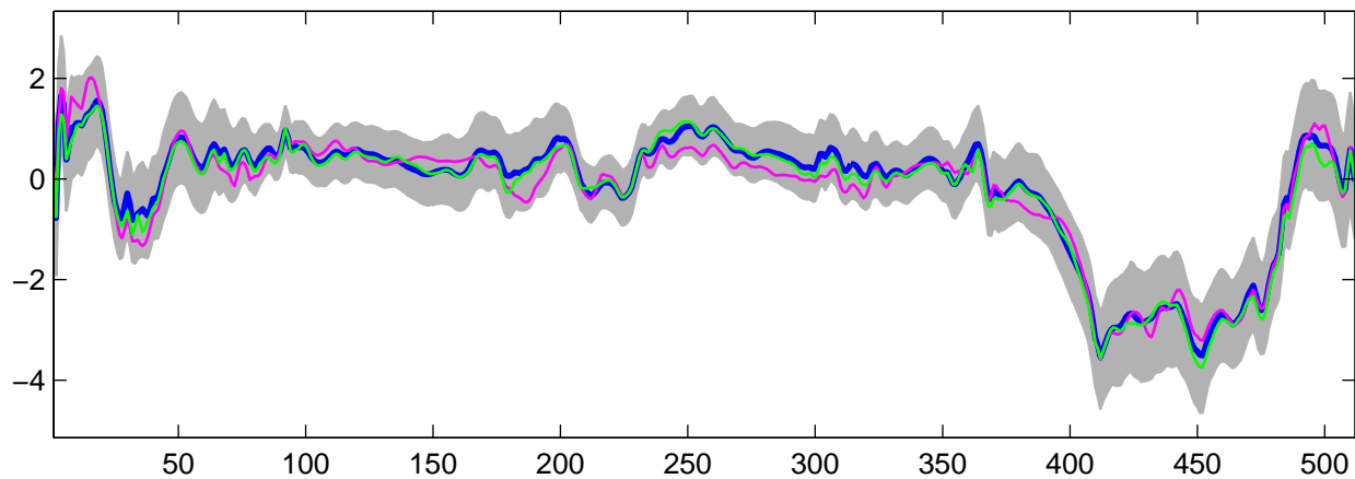
Estimated U_{26}(t) using G-WFMM: DE data, run 10
