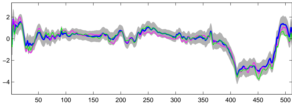
Estimated U_{26}(t) using R-WFMM: DE data, run 10
