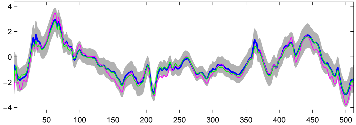
Estimated U_{26}(t) using G-WFMM: Normal data, run 10
