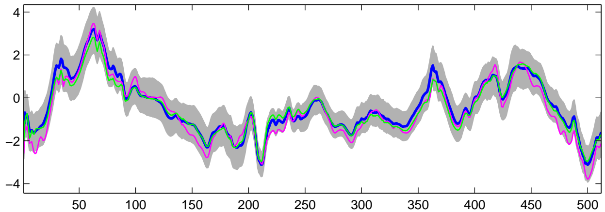
Estimated U_{26}(t) using R-WFMM: Normal data, run 10
