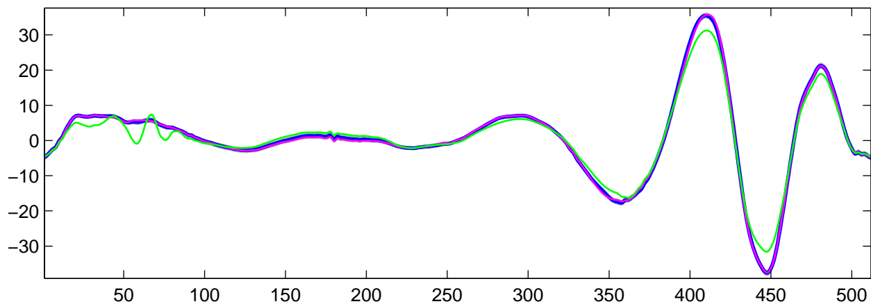
Estimated U_{26}(t) using R-WFMM: t_1 data, run 10
