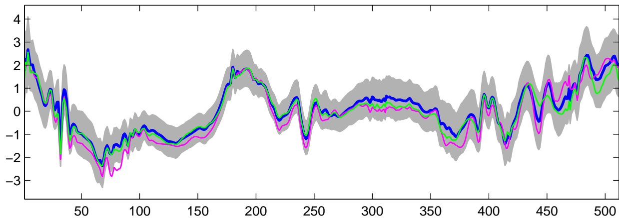
Estimated U_{26}(t) using G-WFMM: t_2 data, run 10
