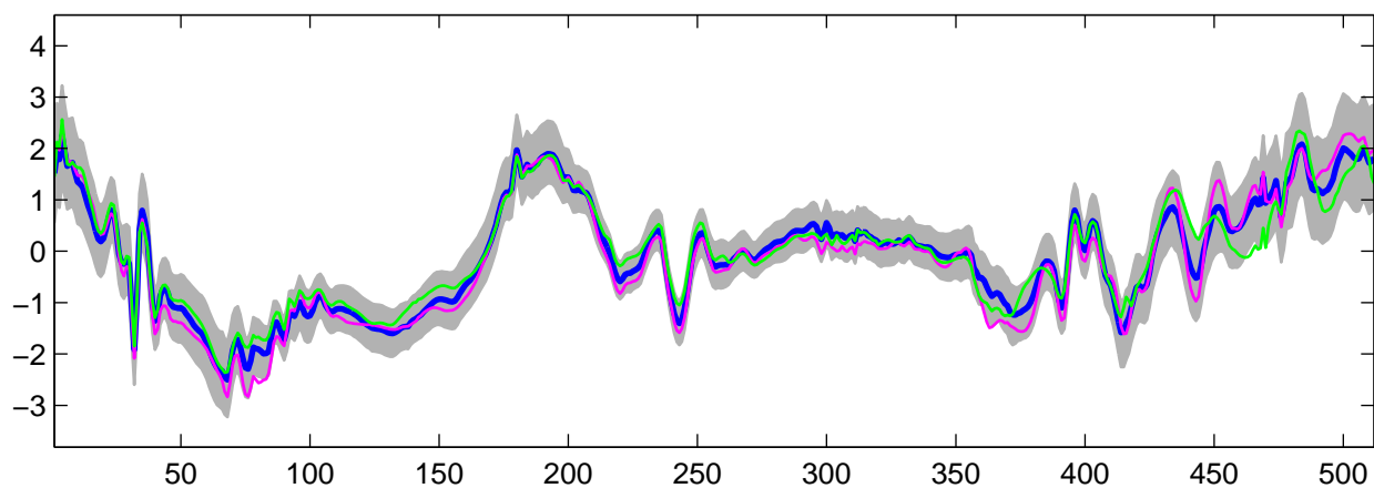
Estimated U_{26}(t) using R-WFMM: t_2 data, run 10
