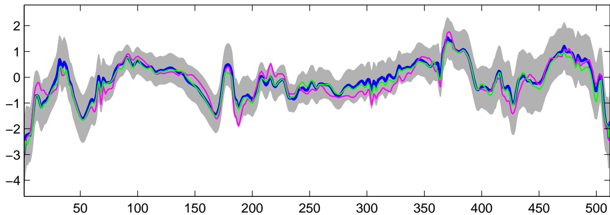
Estimated U_{27}(t) using G-WFMM: DE data, run 10
