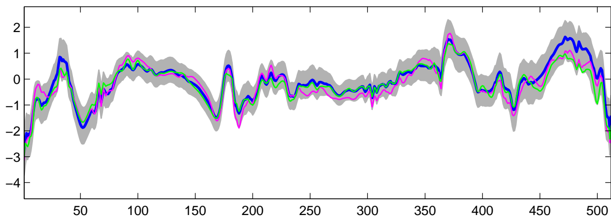
Estimated U_{27}(t) using R-WFMM: DE data, run 10
