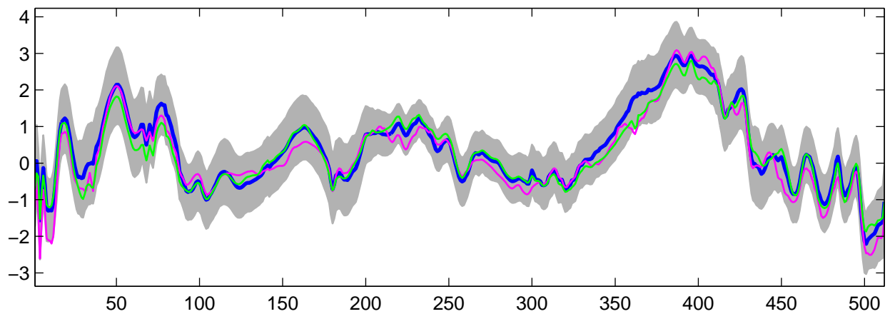
Estimated U_{27}(t) using R-WFMM: Normal data, run 10
