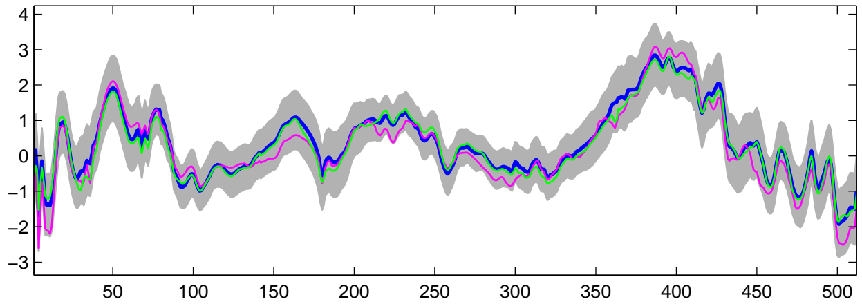
Estimated U_{27}(t) using G-WFMM: Normal data, run 10
