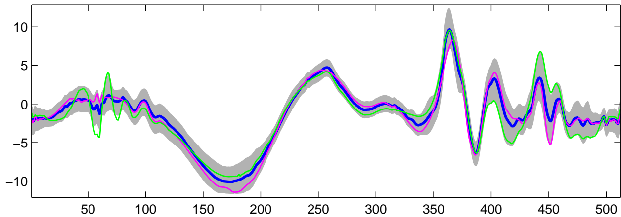
Estimated U_{27}(t) using G-WFMM: t_1 data, run 10
