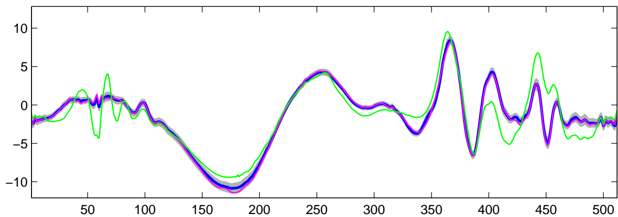
Estimated U_{27}(t) using R-WFMM: t_1 data, run 10
