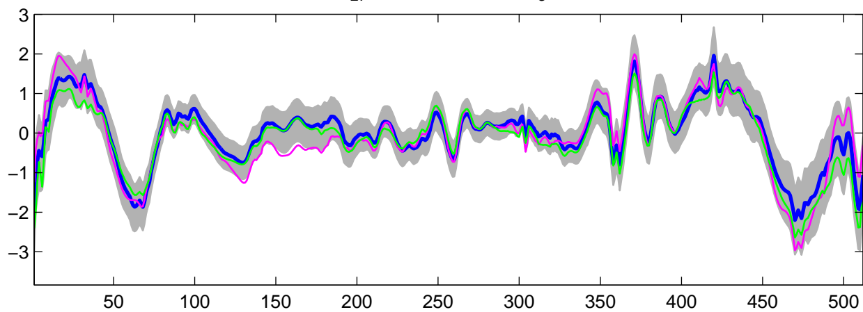
Estimated U_{27}(t) using R-WFMM: t_3 data, run 10
