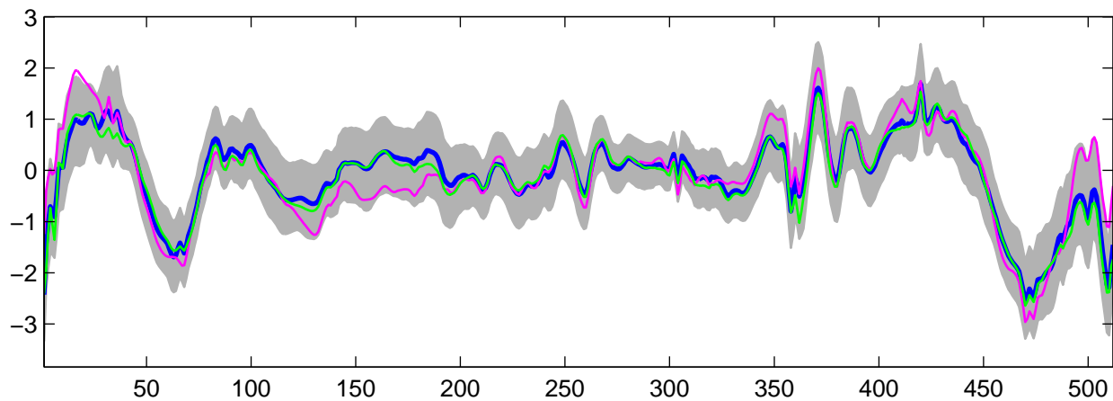
Estimated U_{27}(t) using G-WFMM: t_3 data, run 10
