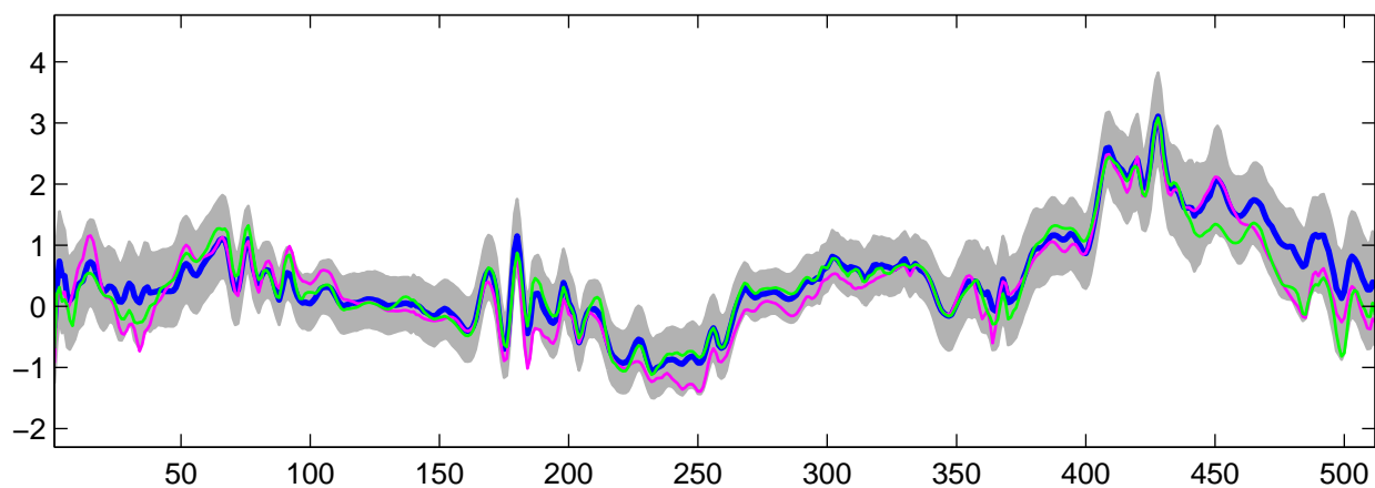
Estimated U_{28}(t) using R-WFMM: DE data, run 10
