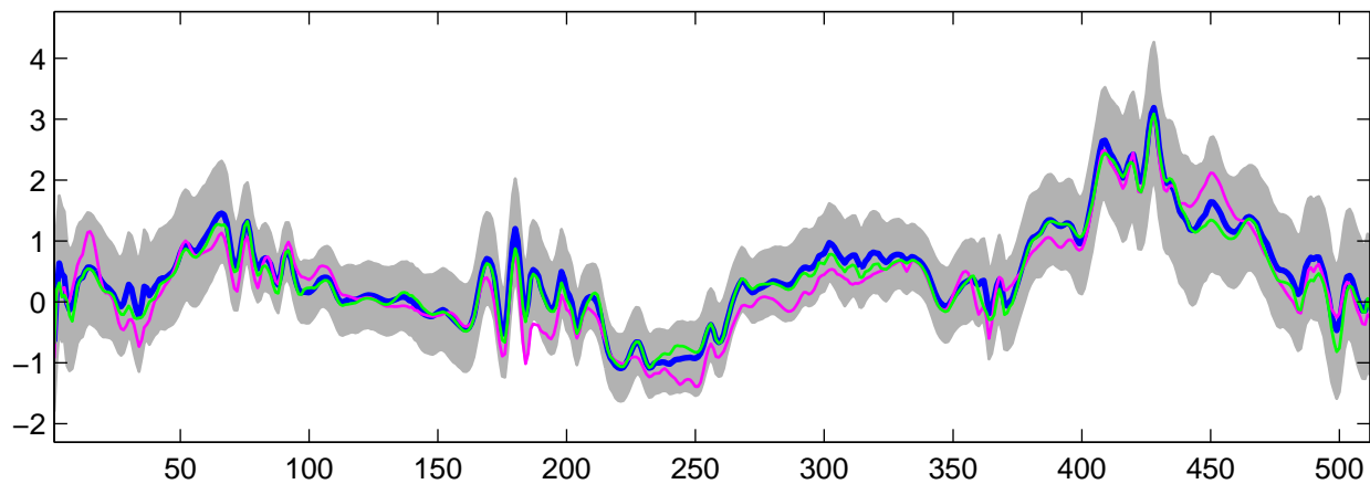
Estimated U_{28}(t) using G-WFMM: DE data, run 10
