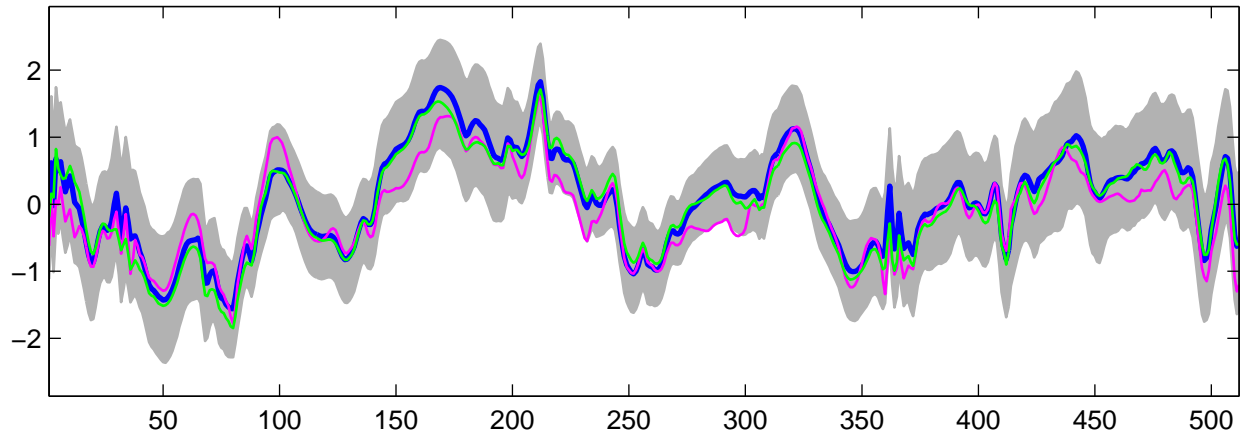
Estimated U_{28}(t) using G-WFMM: Normal data, run 10
