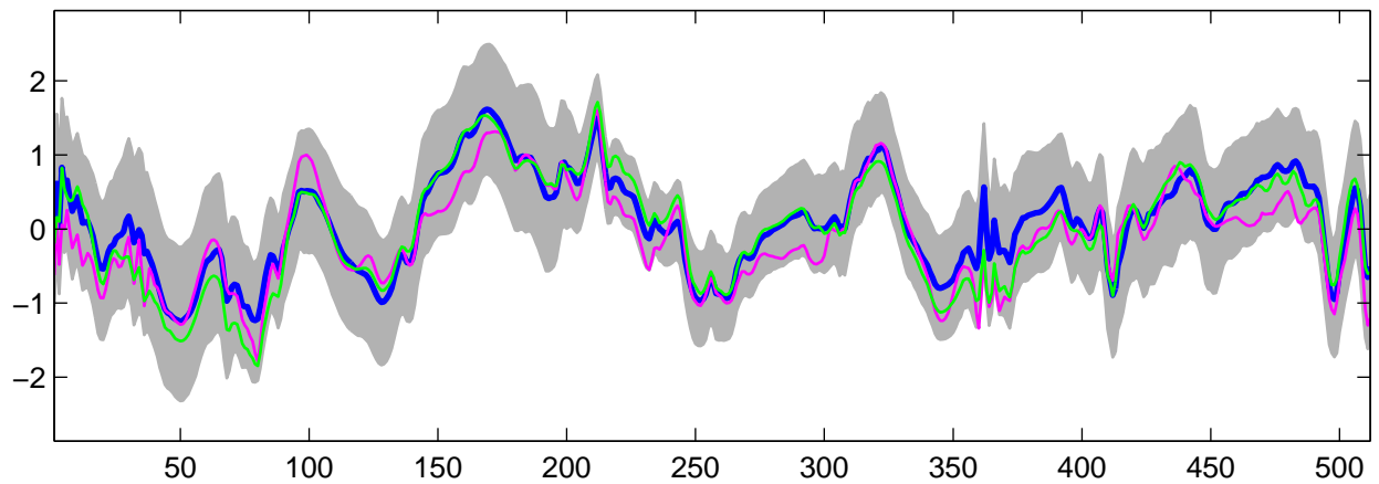
Estimated U_{28}(t) using R-WFMM: Normal data, run 10
