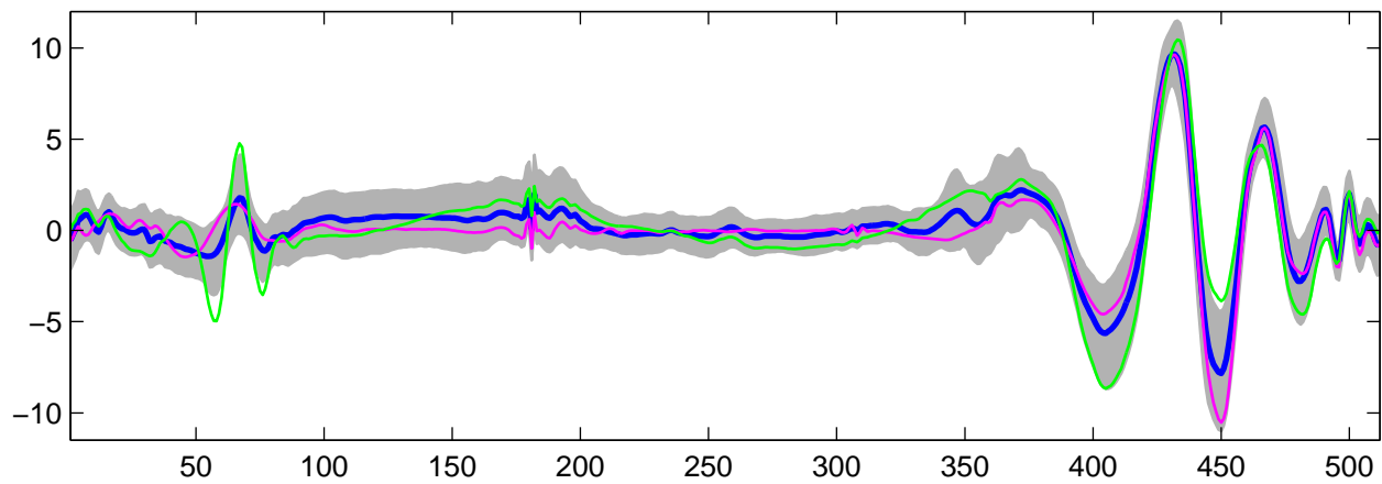
Estimated U_{28}(t) using G-WFMM: t_1 data, run 10
