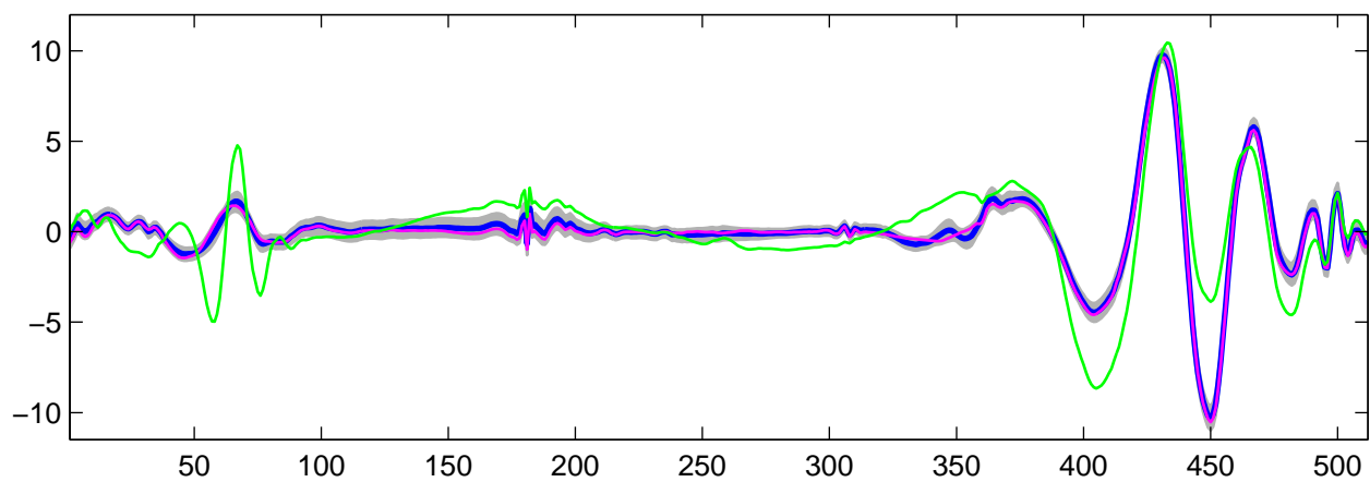
Estimated U_{28}(t) using R-WFMM: t_1 data, run 10
