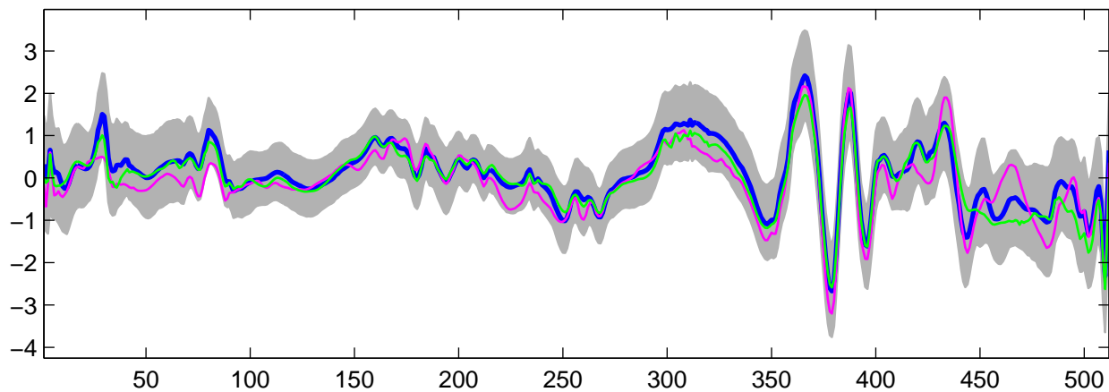
Estimated U_{28}(t) using G-WFMM: t_2 data, run 10
