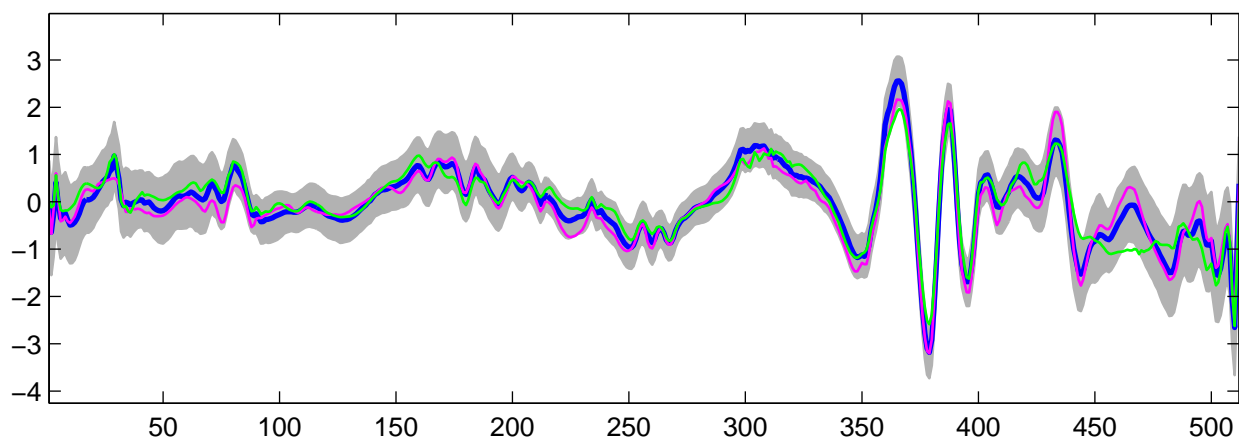
Estimated U_{28}(t) using R-WFMM: t_2 data, run 10
